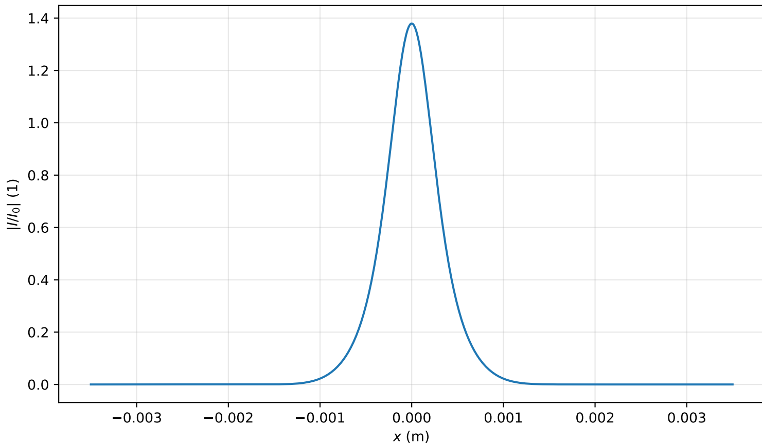
Intensity profile I(x, y = 0, z = 0.796m)/I_0 , P_{in}=1.0P_{cr} , artificial time
